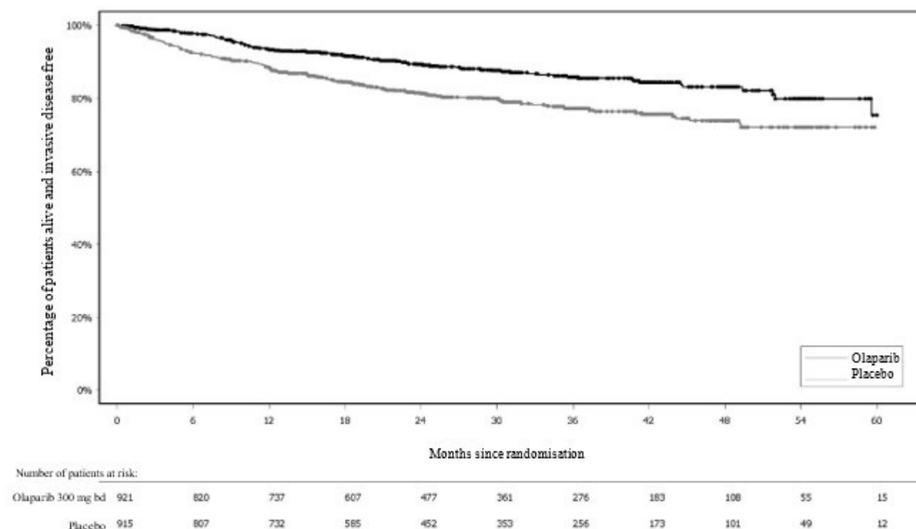
Figure 9 Kaplan-Meier plot of IDFS for adjuvant treatment of patients with germline BRCA -mutated high risk early breast cancer in OlympiA (DCO 27 March 2020)
