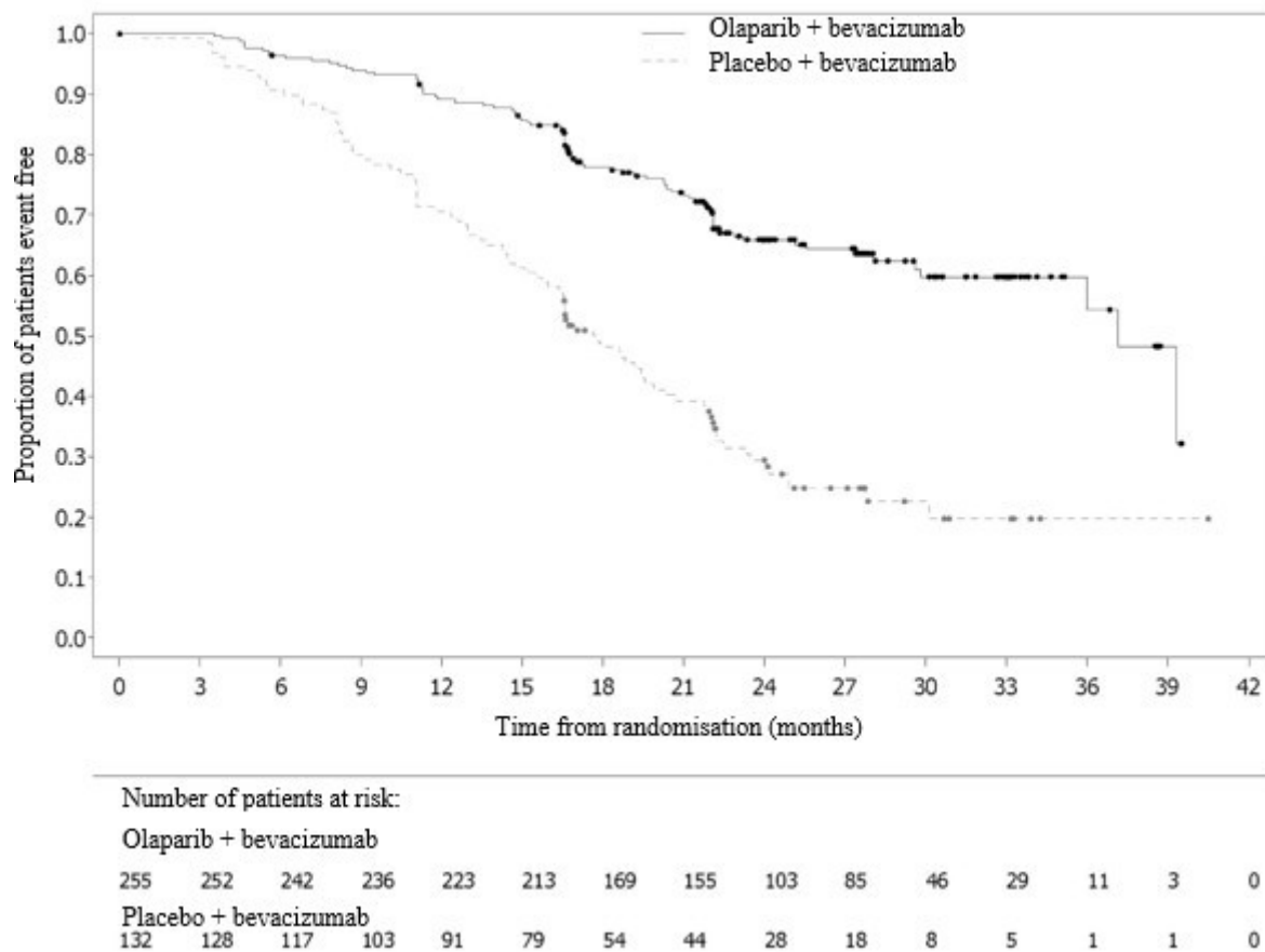
Figure 8 PAOLA-1: Kaplan-Meier Plot, Final Overall Survival by HRD Status Positive (including tBRCAm) (DCO 22 March 2022)
