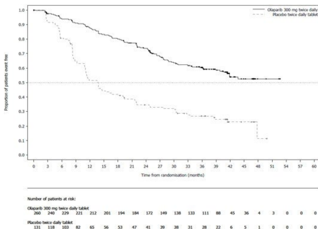
Figure 1 SOLO1: Kaplan-Meier plot of PFS in newly diagnosed patients with BRCA1/2m advanced ovarian cancer (51% maturity - investigator assessment)
