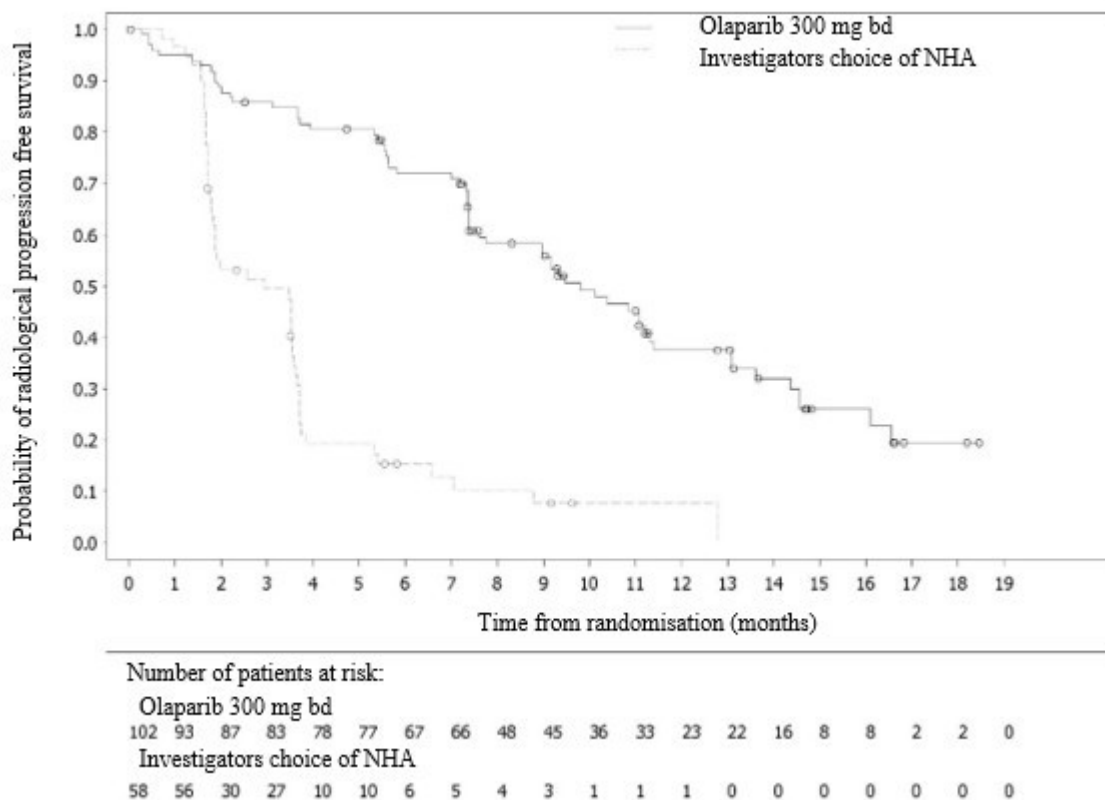
Figure 16 BRCA1/2m patients: Kaplan-Meier plot of rPFS (by BICR)
