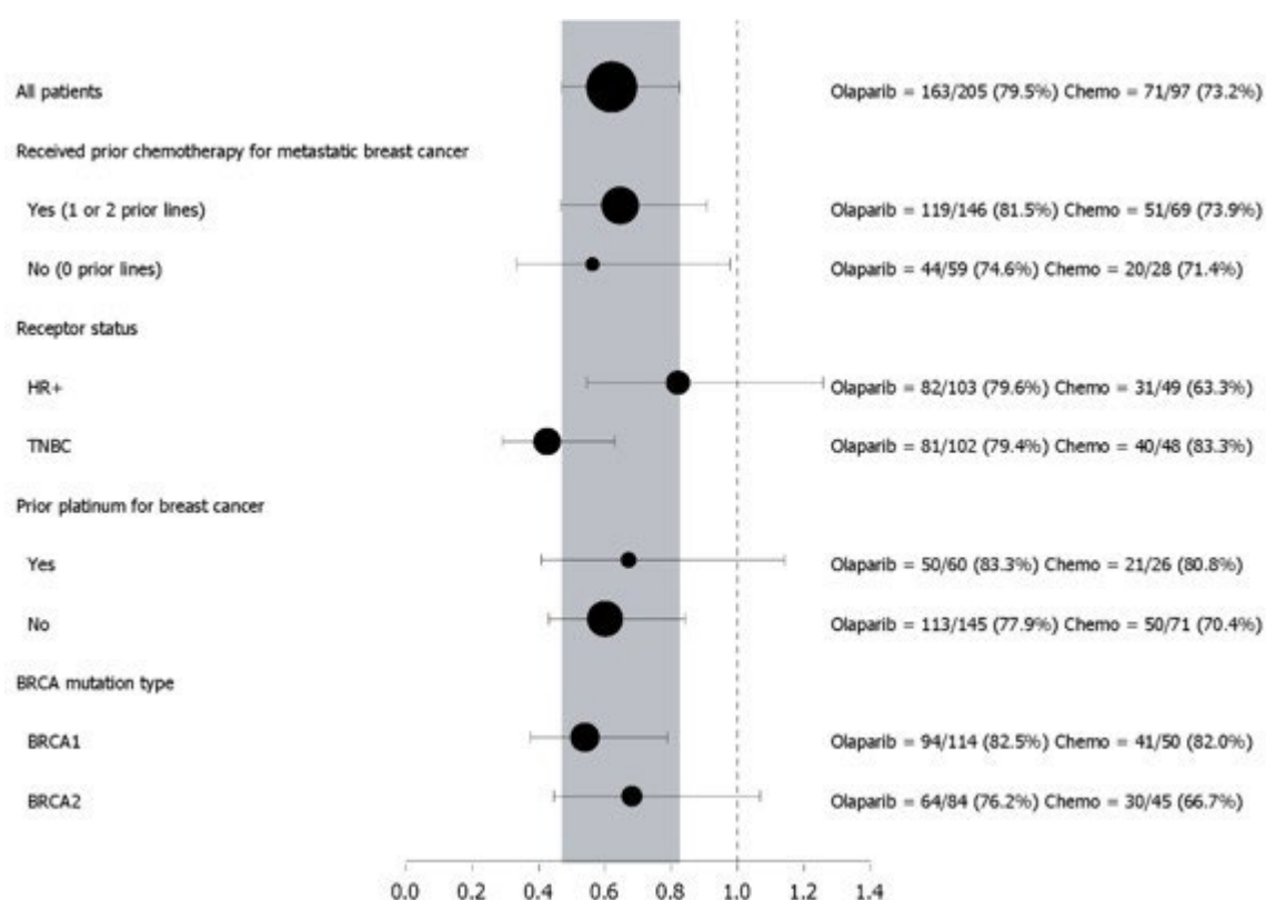
Figure 12 PFS (BICR), Forest plot, by prespecified subgroup
