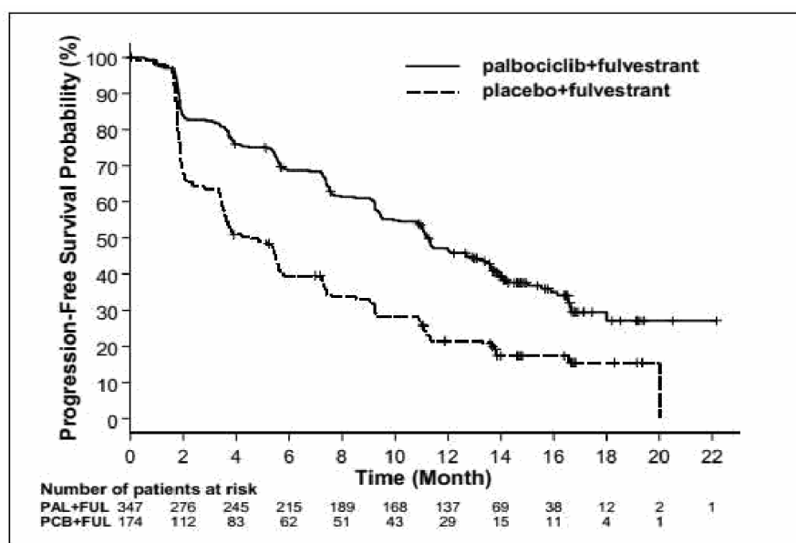
Figure 2. Kaplan-Meier plot of progression-free survival (investigator assessment, intent-to-treat population) – PALOMA-3 study (23 October 2015 cutoff)
