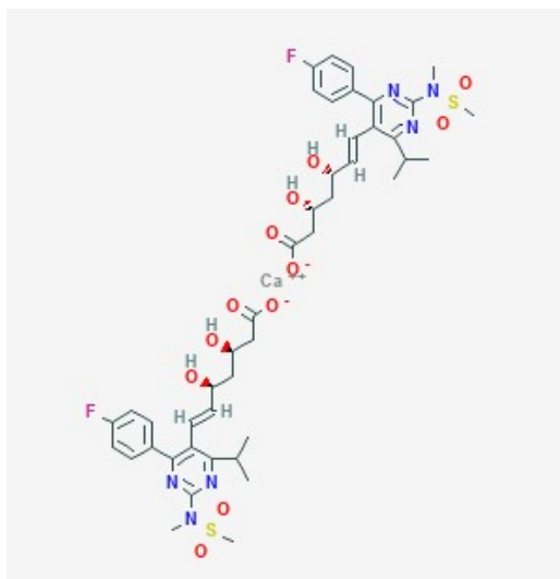
STRUCTURAL FORMULA: ROSUVASTATIN CALCIUM
